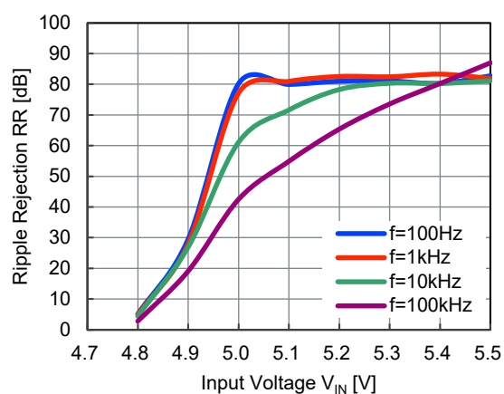
NR1640DC480x, I_{OUT} = 50\text{ mA}
