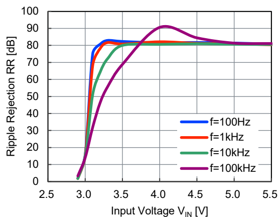
NR1640DC290x, I_{OUT} = 100\text{ mA}
