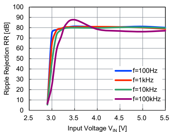
NR1640DC290x, I_{OUT} = 10\text{ mA}
