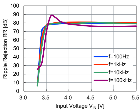
NR1640DC330x, I_{OUT} = 1\text{ mA}
