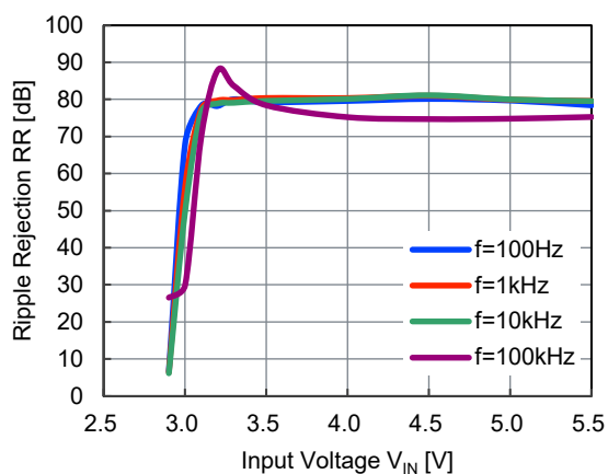
NR1640DC290x, I_{OUT} = 1\text{ mA}
