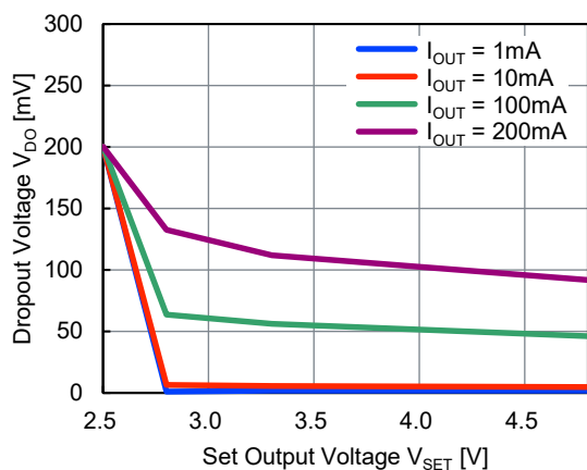
4) Dropout Voltage vs Set Output Voltage
