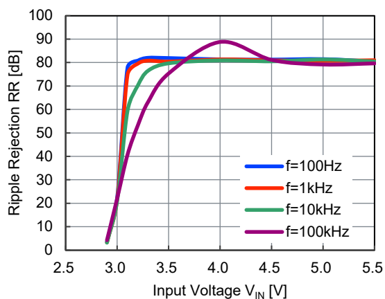
NR1640DC290x, I_{OUT} = 50\text{ mA}
