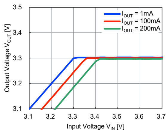
NR1640DC330x, ( V_{IN}=3.1V to 3.7V )
