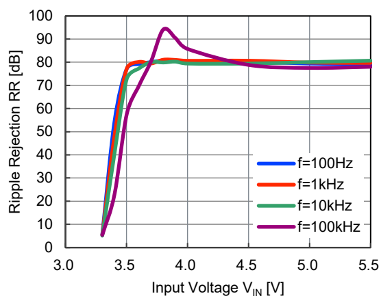
NR1640DC330x, I_{OUT} = 10\text{ mA}
