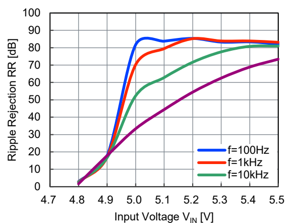
NR1640DC480x, I_{OUT} = 100\text{ mA}
