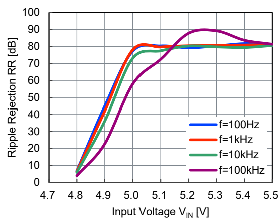
NR1640DC480x, I_{OUT} = 10\text{ mA}
