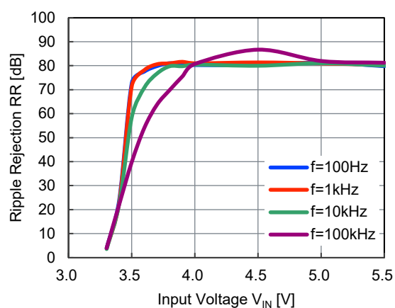
NR1640DC330x, I_{OUT} = 50\text{ mA}
