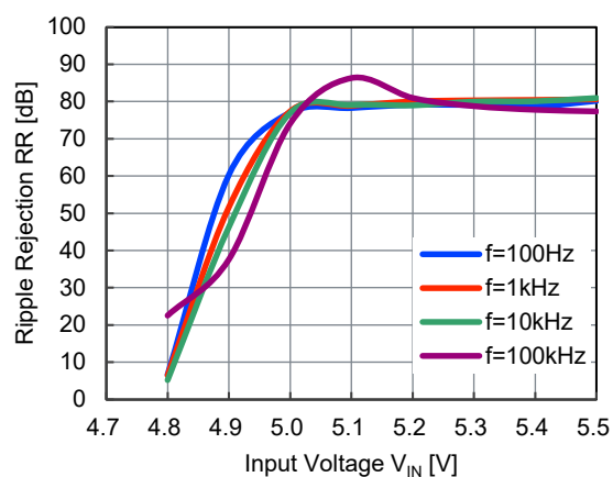
NR1640DC480x, I_{OUT} = 1\text{ mA}
