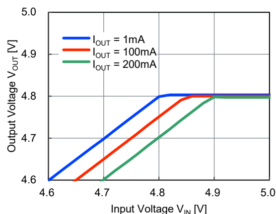
NR1640DC480x, ( V_{IN}=4.6V to 5.5V )
