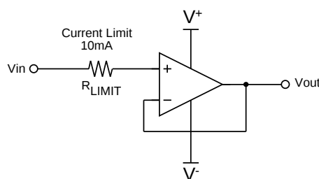
Figure 6. Example of input protection
