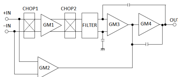
Figure 1. Functional block
