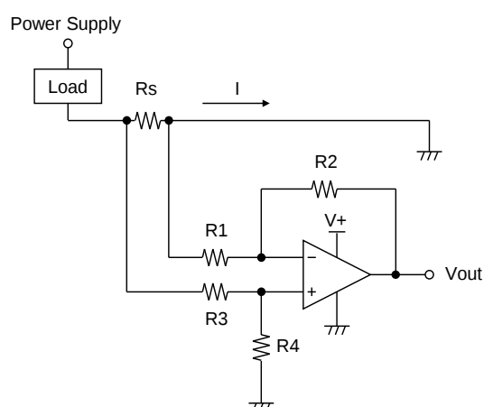
Figure14. Low-Side Current Sensing
