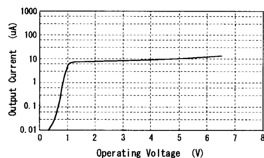
Output Current vs. Operating Voltage VIN=0.1V
