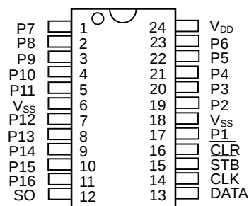
NJU3716AM, NJU3716AVC2
