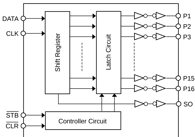
NJU3716AM, NJU3716AVC2
