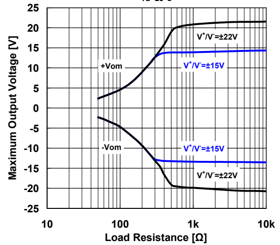
Maximum Output Voltage vs. Load Resistance T_a=25^\circ\text{C}
