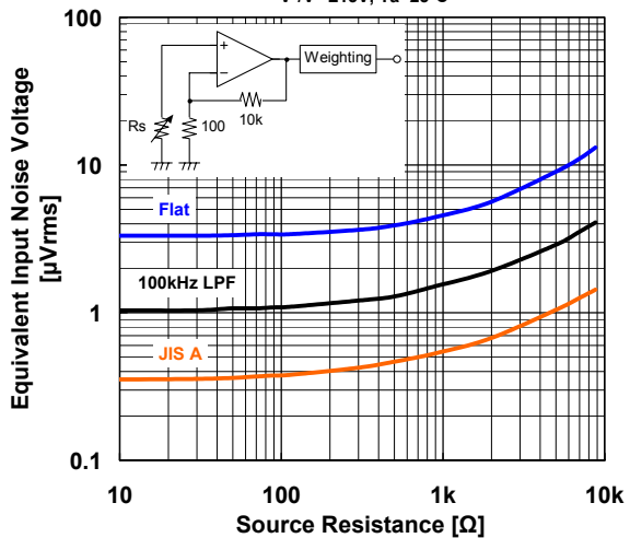
Voltage Noise vs. Source Resistance V^+/V^-=\pm 15\text{V} , T_a=25^\circ\text{C}
