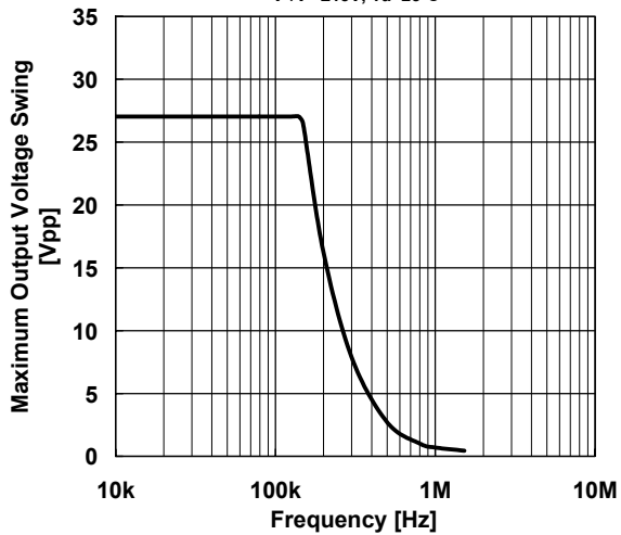
Maximum Output Voltage Swing vs. Frequency V^+/V^-=\pm 15\text{V} , T_a=25^\circ\text{C}
