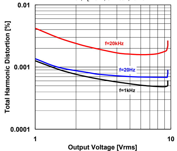
THD vs. Output Voltage
