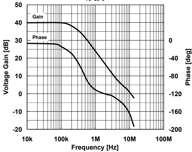
Gain/Phase vs. Frequency T_a=25^\circ\text{C}
