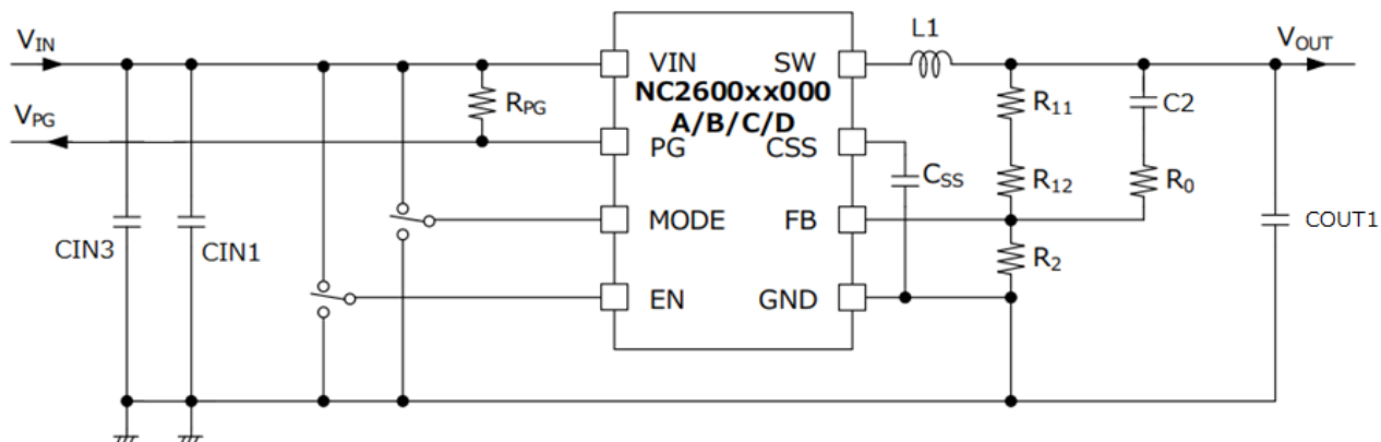
NC2600xx Typical Application Circuit
