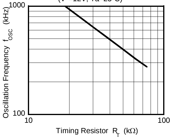
Timing Resistor vs.Oscillation Frequency ( V^+=12\text{V} , T_a=25^\circ\text{C} )
