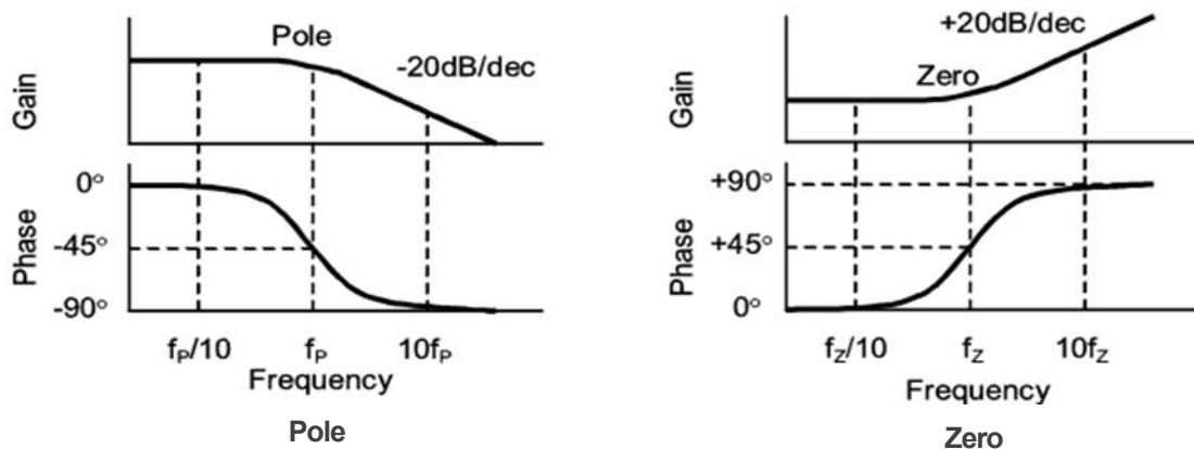
Figure 9. Pole and Zero Characteristics
