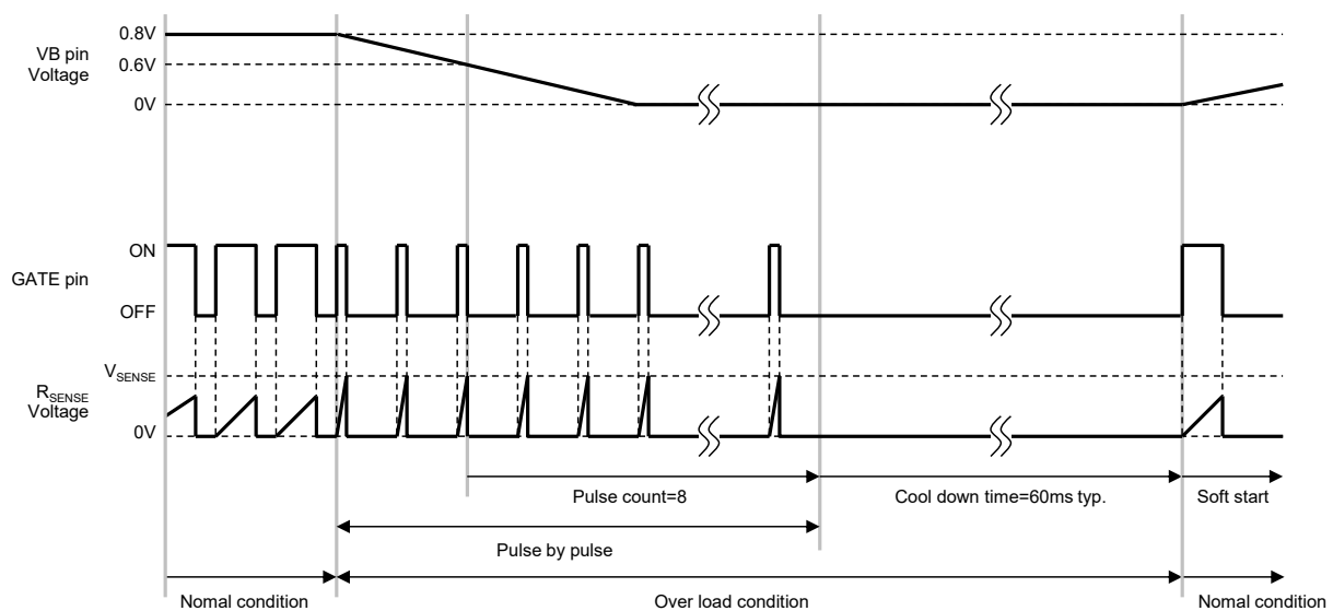
Figure 4. OCP Timing Chart
