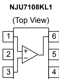
NJU7108KL1 PIN CONFIGURATION 1. +INPUT 2. V_{SS} 3. -INPUT 4. V_{DD} 5. V_{SS} 6. OUTPUT
