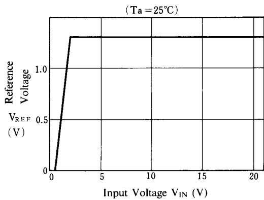
Reference Voltage
