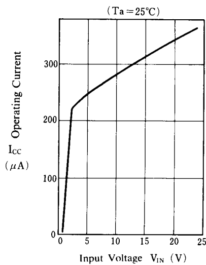
Operating Current
