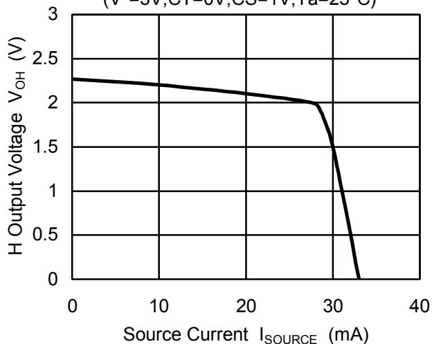
H Output Voltage(OUT Pin) vs. Source Current ( V^+=3V, C_T=0V, C_S=1V, T_a=25^\circ C )
