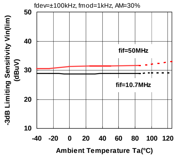
-3dB Limiting Sensitivity versus Temperature
