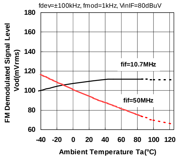
Demodulated Signal Level versus Temperature
