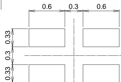
PCB Pattern
