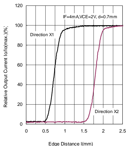
Output Current vs. Edge Distance IR LED(Ta=25°C)
