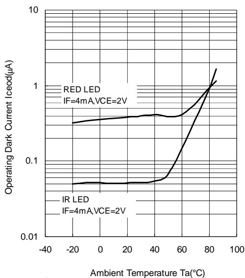
Operating Dark Current vs. Temperature RED LED & IR LED
