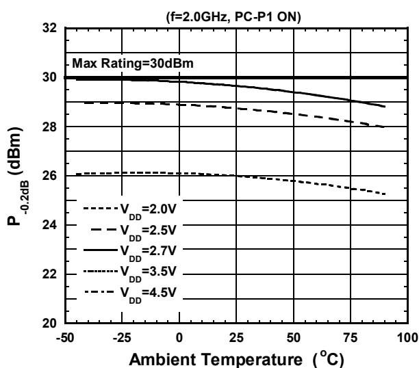
P_{-0.2\text{dB}} vs Temperature
