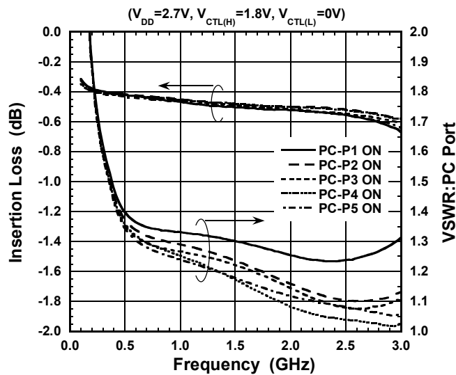
Loss, VSWR vs Frequency
