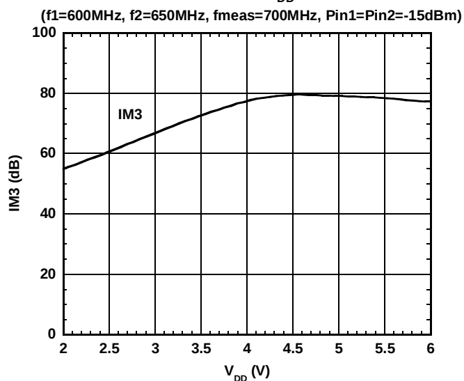
IM3 vs. V_{DD}
