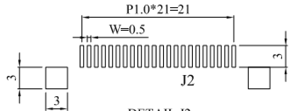
DETAIL J2 SCALE 2/1
