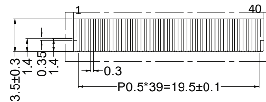
DETAIL A
