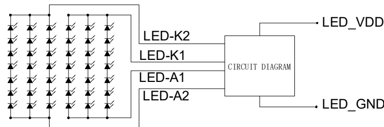
Backlight Circuit
