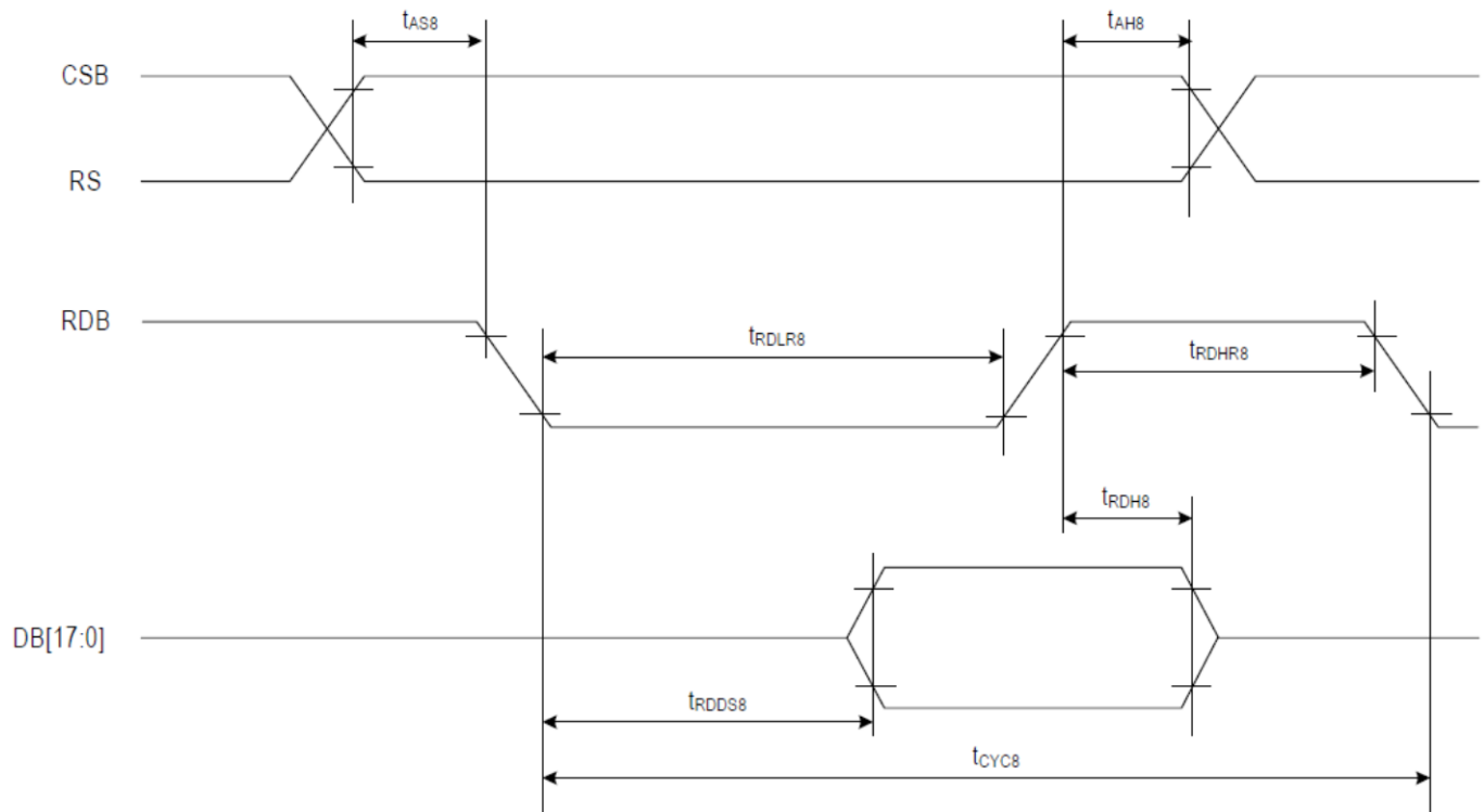
( Read Timing )
