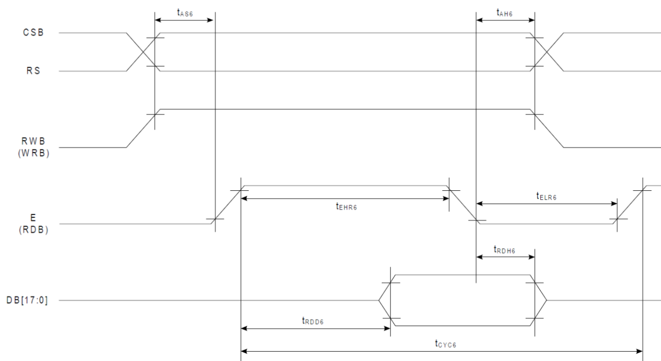
( Read Timming )
