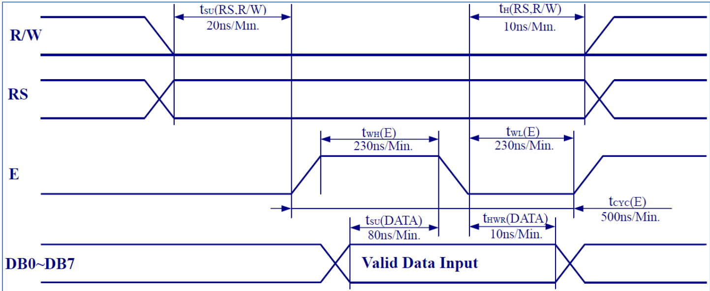
M68 Write Timing:
