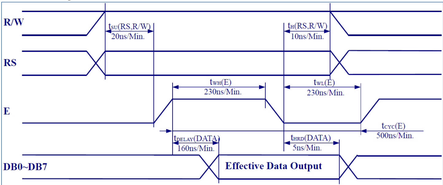
M68 Read Timing:
