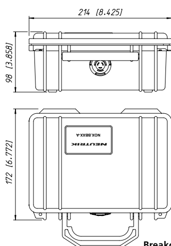
Breakout Box
