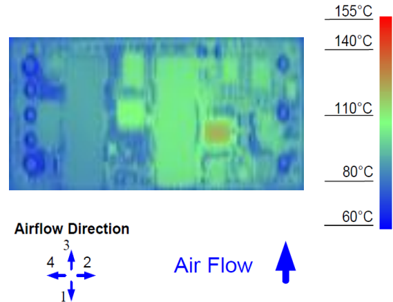
Figure 12. Thermal Image for Airflow Direction 3 (4.2A output, 85°C ambient, 200 LFM, typical Vin, open frame, socket interface)
