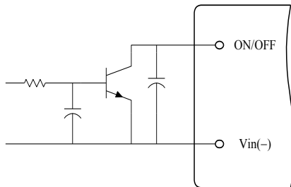
Fig. 14 Open Collector Enable Circuit
