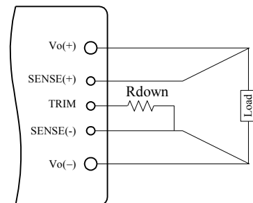
Fig. 16 Circuit to Decrease Output Voltage
