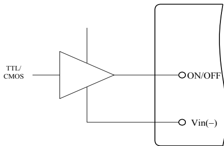
Fig. 15 Direct Logic Drive
