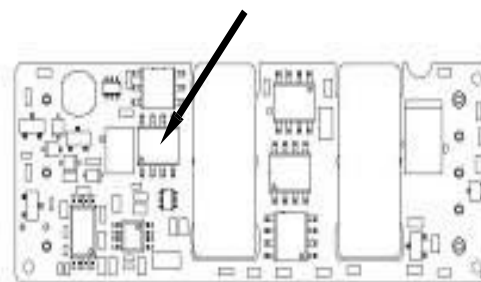
Figure 18. Temperature Monitoring Location
