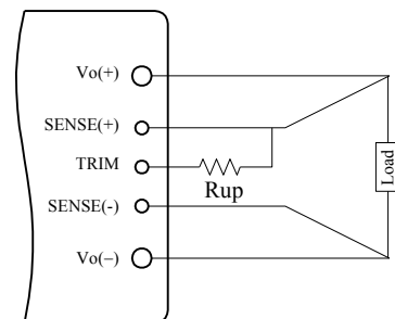
Fig. 17 Circuit to Increase Output Voltage
