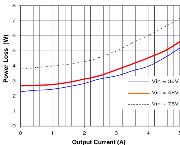
Figure 2. Power Loss vs. Load Current (25°C)
