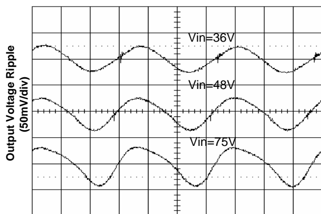
Figure 5. Output Voltage Ripple at Full Load
