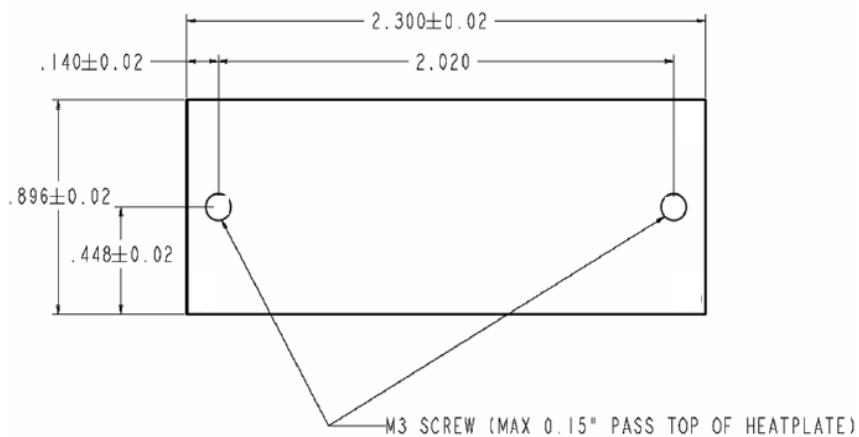
Figure 20. Converter with optional baseplate
