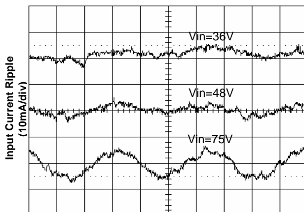
Figure 6. Input Reflected Ripple at Full Load
