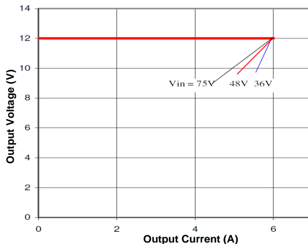
Figure 10. Output Characteristics
