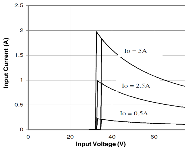
Figure 9. Input Characteristics
