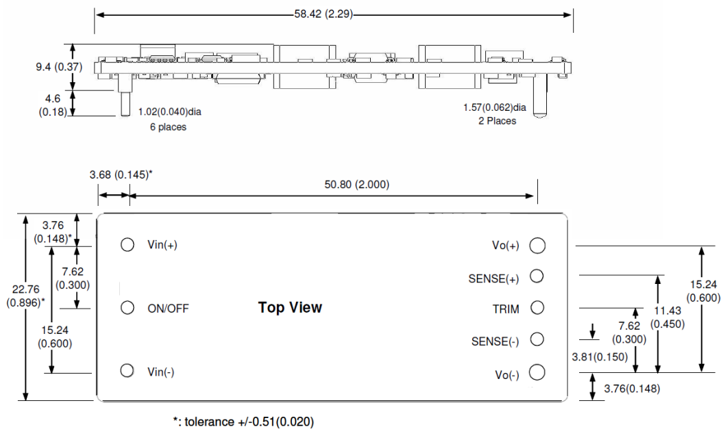
Figure 19. Converter with Open frame option
