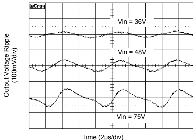
Figure 4. Output Ripple Voltage at Full Load
