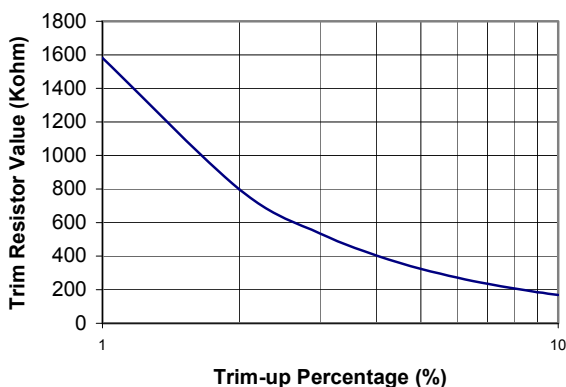
Figure 13. Trim-Up Resistor Selection
