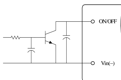
Figure 10. Open Collector Enable Circuit
