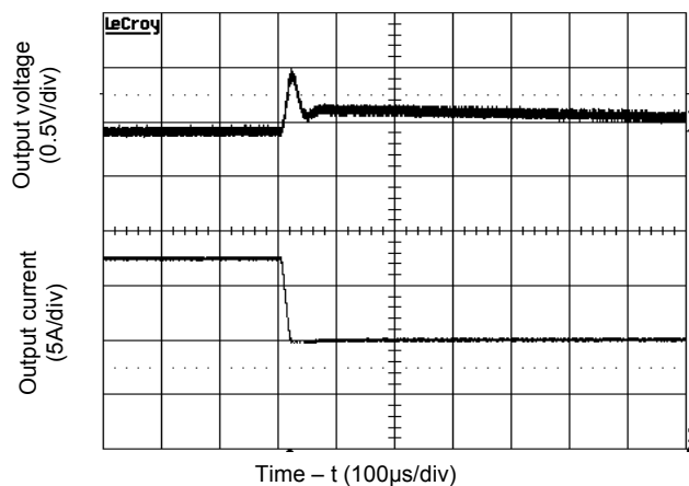
Figure 5. Transient Load Response (Typical Vin, 75% to 50% full load step at a slew rate 0.1A/μs)
