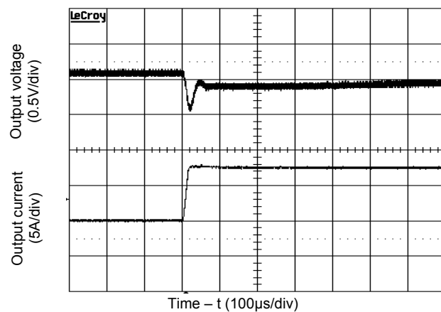
Figure 6 Transient Load Response (Typical Vin, 50% to 75% full load step at a slew rate 0.1A/μs)
