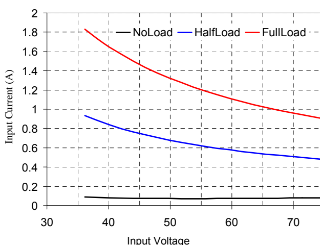
Figure 2. Input Characteristics
