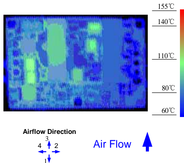
Figure 12. Thermal Image for Airflow Direction 3 (7A output, 55°C ambient, 200 LFM, typical Vin, open frame unit using soldering interface)
