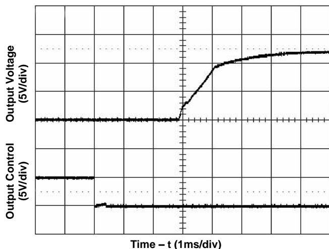
Figure 3. Start-Up from Enable Control Input voltage 24V, Output current 7A
