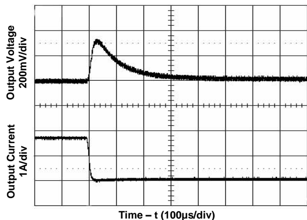
Figure 7. Transient Load Response
