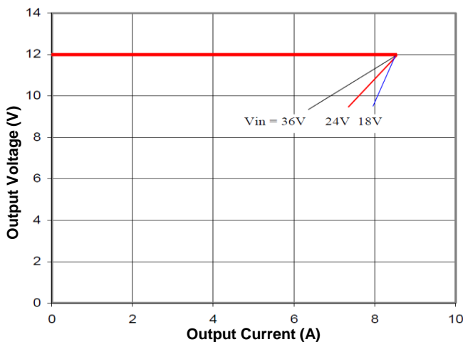
Figure 10. Output Characteristics
