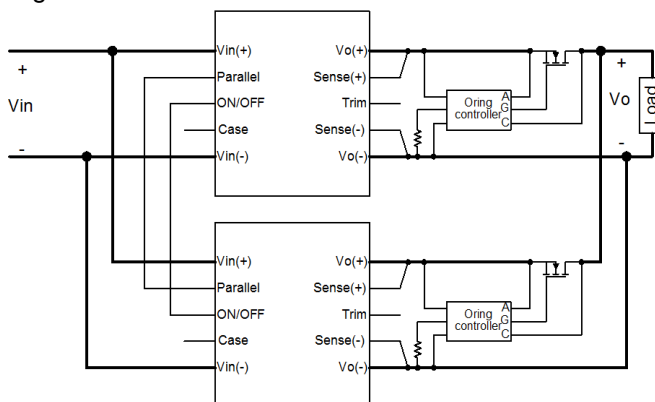
Figure 19. Circuit Configuration for Active Current Share
