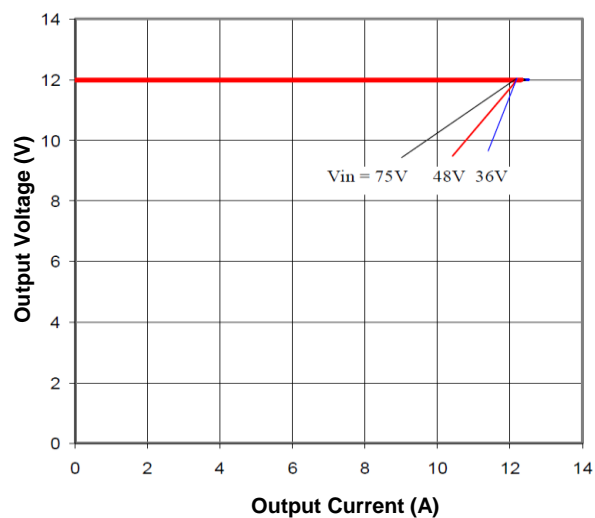
Figure 10. Output Characteristics
