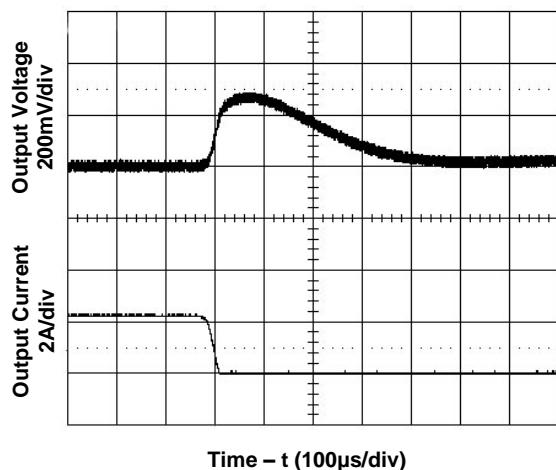
Figure 7. Transient Load Response Top: Output voltage deviation Bottom: Load current step (-25% full load) Test Cond.: Output current at 20A 50% full load typical Vin, slew rate 0.1A/μs
