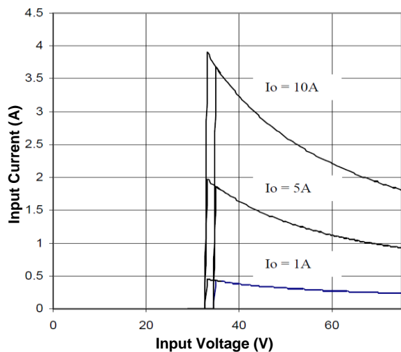
Figure 9. Input Characteristics
