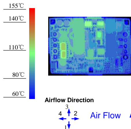
Figure 12. Thermal Image for Airflow Direction 3 (8.4A output, 55 ^{\circ}C ambient, 200 LFM, typical V_{in} , open frame unit using soldering interface)
