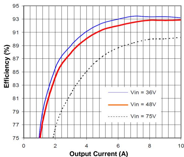
Figure 1. Efficiency vs. Load Current ( 25^\circ\text{C} )
