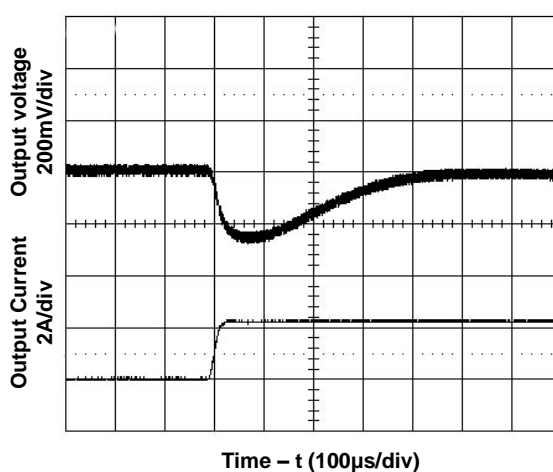
Figure 8. Transient Load Response Top: Output voltage deviation Bottom: Load current step (+25% full load) Test Cond.: Output current at 20A 50% full load, typical Vin, slew rate 0.1A/μs
