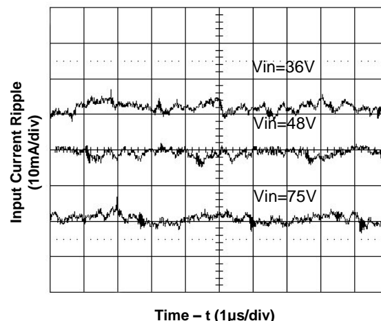
Figure 6. Input Reflected Ripple Current at Full Load
