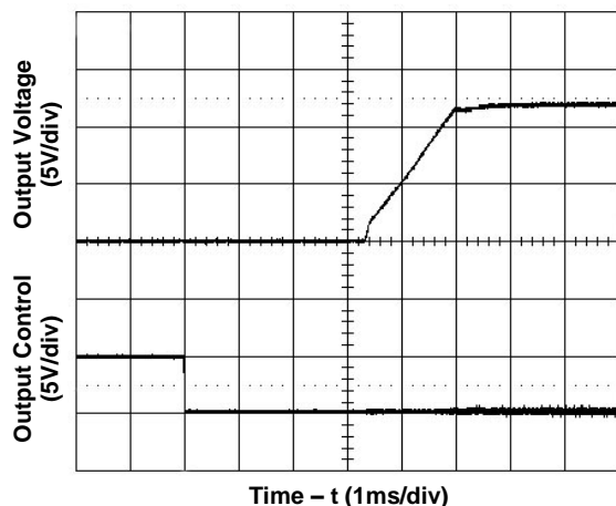
Figure 3. Start-Up from Enable Control (Input voltage 48V, Output current 10A)
