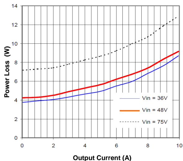
Figure 2. Power Loss vs. Load Current ( 25^\circ\text{C} )
