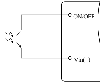
Figure 10. Opto Coupler Enable Circuit
