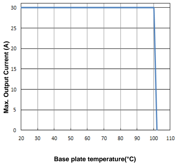
Figure 9. Current Derating Curve for Base plate (typical vin with Base plate; solder interface)
