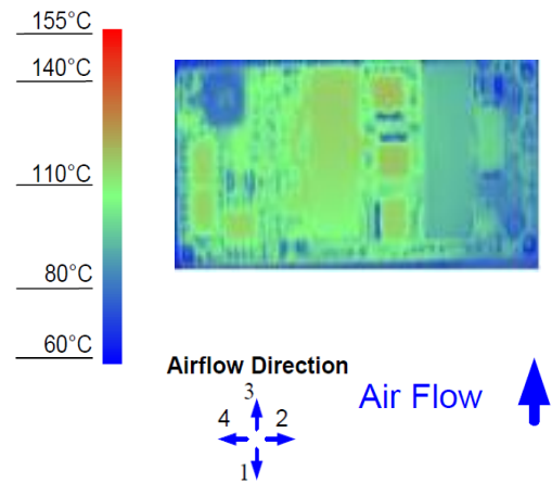
Figure 8. Thermal Image for Airflow Direction 3 (30A output, 55°C ambient, 200 LFM, typical Vin, open frame, socket interface)
