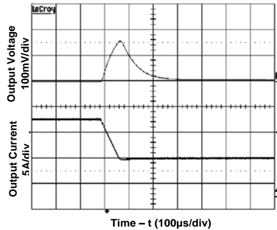
Figure 6. Transient Load Response (Typical Vin, load current steps from 50% to 75% at a slew rate 0.1A/μs)
