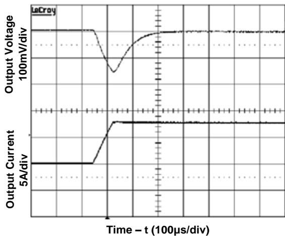
Figure 5. Transient Load Response (Typical Vin, load current steps from 50% to 25% at a slew rate 0.1A/μs)
