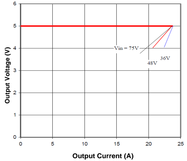
Figure 10. Output Characteristics
