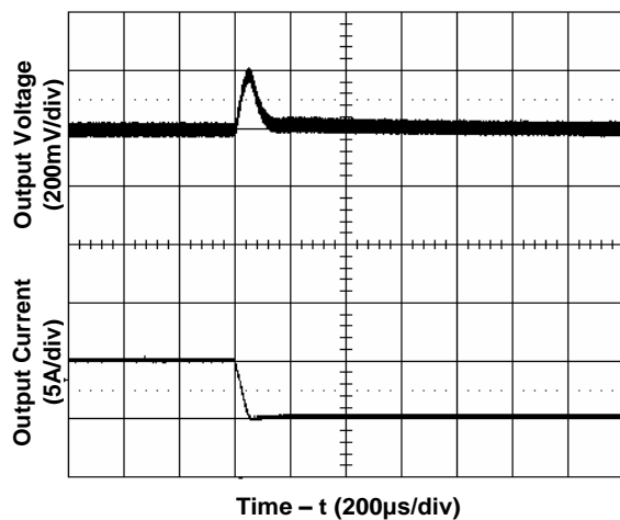
Figure 7. Transient Load Response (Typical Vin, load current steps from 50% to 25% at a slew rate 0.1A/μs)
