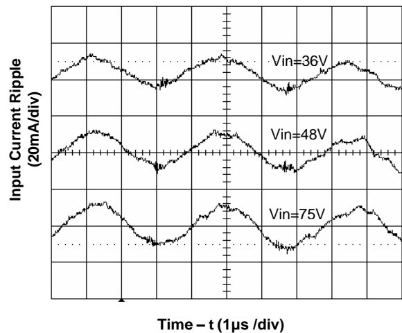
Figure 6. Input Reflected Ripple at Full Load
