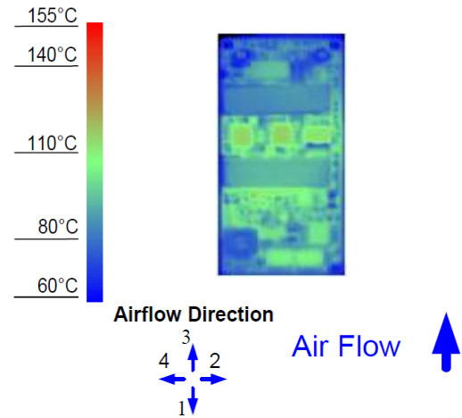
Figure 12. Thermal Image for Airflow Direction 2 (18.7A output, 55 ^{\circ}C ambient, 200 LFM, typical V_{in} , open frame, socket interface)
