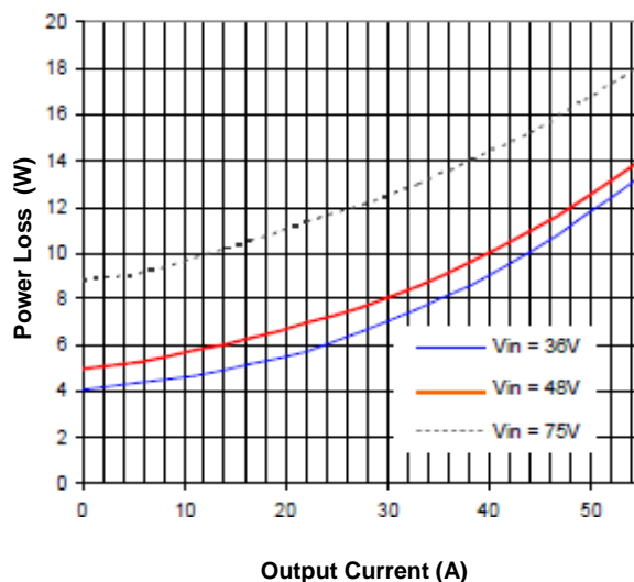
Figure 2. Power Loss vs. Load Current ( 25^\circ\text{C} )
