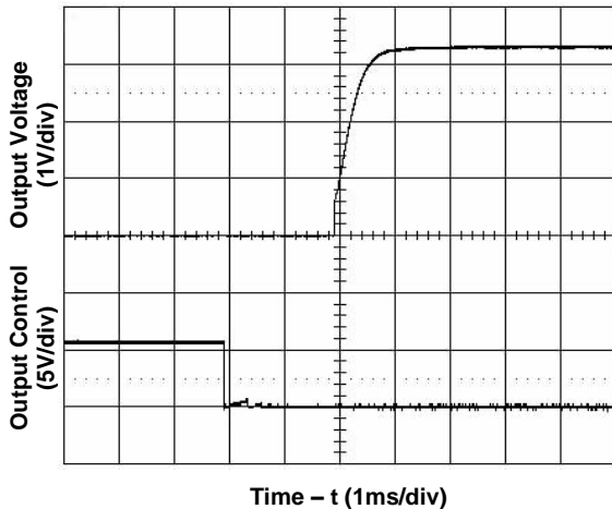
Figure 3. Start-Up from Enable Control Typical Vin, full load (resistive)
