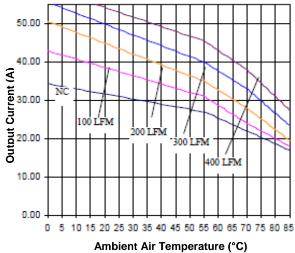
Figure 13. Current Derating Curve for Airflow Direction 2 (Ref. Figure 14 for Airflow Direction; typical V_{in} , Unit with baseplate; using soldering interface)
