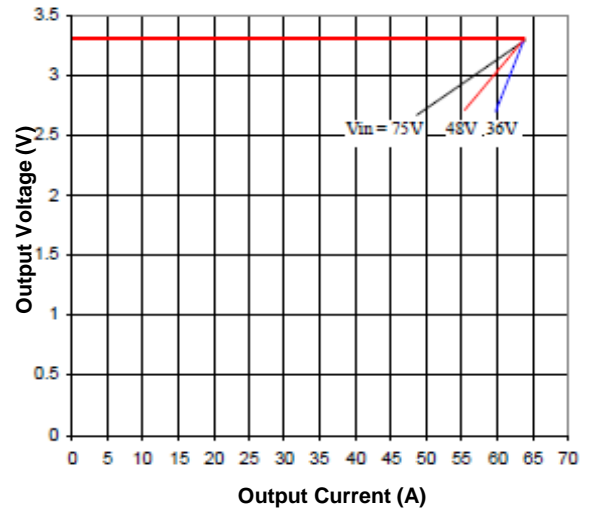
Figure 10. Output Characteristics
