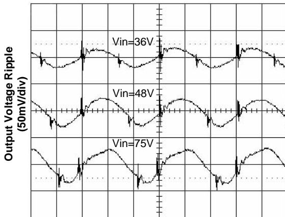
Figure 5. Output Ripple Voltage at Full Load
