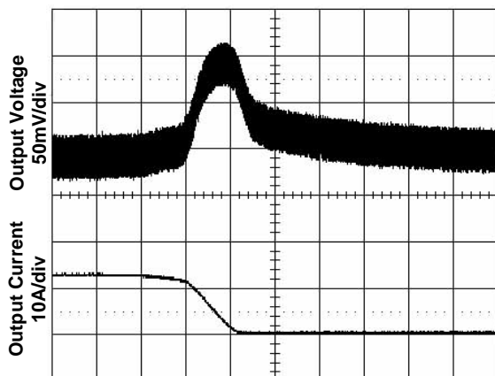
Figure 7. Transient Load Response Top: Output voltage deviation Bottom: Load current step (-25% full load) Test Cond.: Output current at 50% full load, typical Vin, slew rate 0.1A/μs
