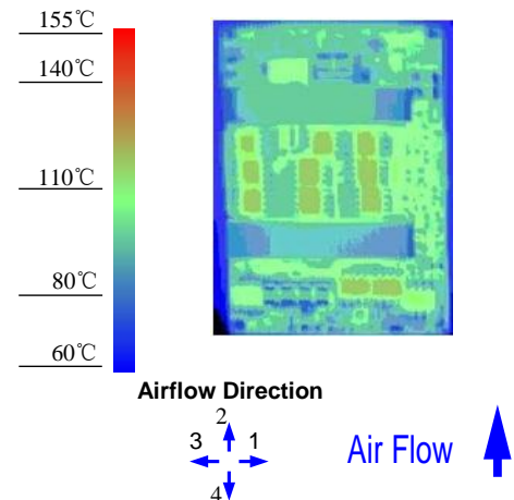
Figure 14. Thermal Image for Airflow Direction 2 (35A output, 55 ^{\circ}C ambient, 200 LFM, V_{in} = 48V open frame unit using solder interface)
