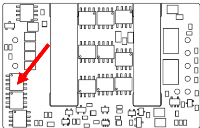
Figure 20. Temperature Monitoring Location
