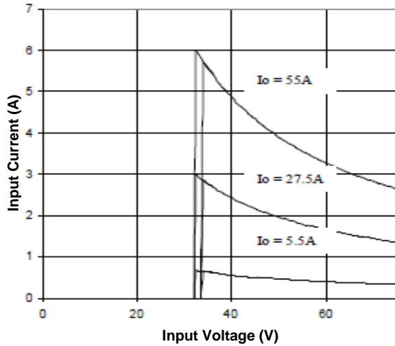
Figure 9. Input Characteristics
