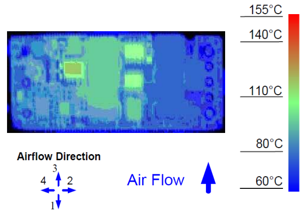
Figure 12. Thermal Image for Airflow Direction 3 (6.4A output, 55°C ambient, 200 LFM, typical Vin, open frame, socket interface)
