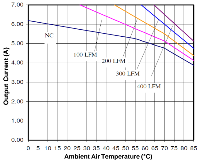
Figure 11. Current Derating Curve for Airflow Direction 3 (Ref. Figure 12 for Airflow Direction; Vin = 48V, open frame unit)
