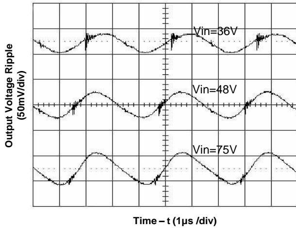
Figure 5. Output Voltage Ripple at Full Load
