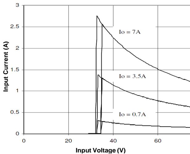
Figure 9. Input Characteristics
