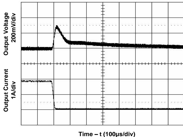
Figure 7. Transient Load Response (Typical Vin, load current steps from 50% to 25% at a slew rate 0.1A/μs)
