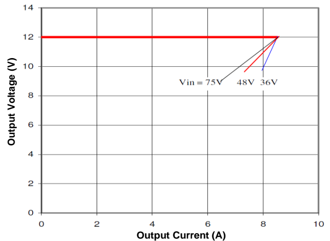
Figure 10. Output Characteristics
