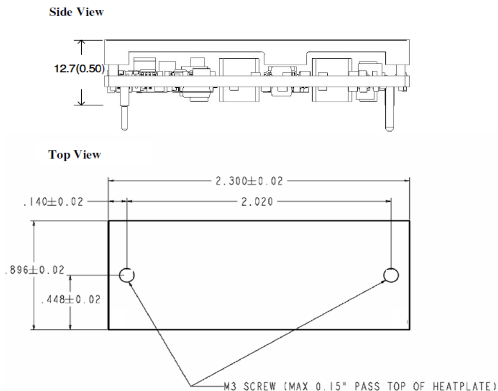
Figure 22. Converter with optional baseplate
