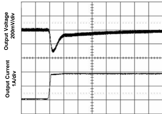
Figure 8. Transient Load Response (Typical Vin, load current steps from 50% to 75% at a slew rate 0.1A/μs)
