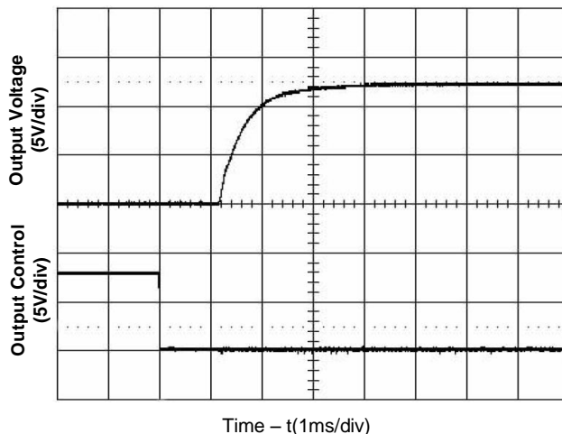
Figure 4. Start-Up from Enable Control (Typical Input voltage and zero load)
