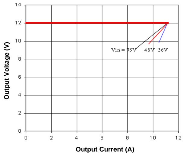
Figure 10. Output Characteristics
