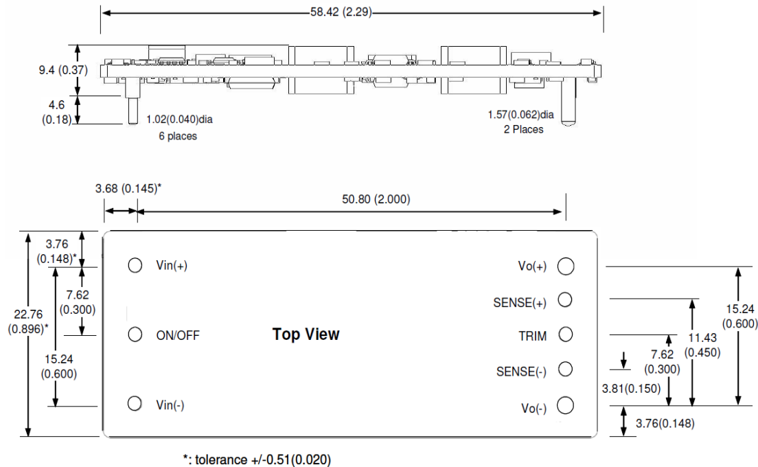
Figure 21. Converter with Open frame option
