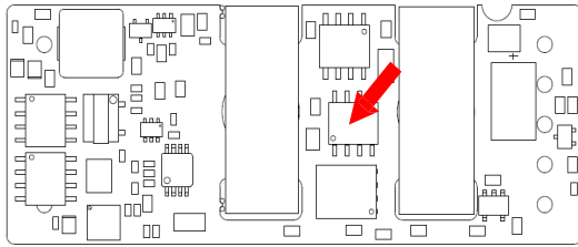
Figure 20. Temperature Monitoring Location
