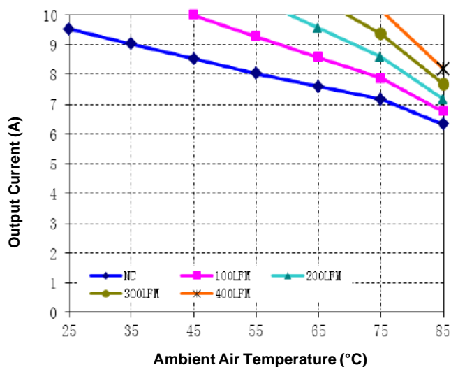
Figure 13. Current Derating Curve for Airflow Direction 2 (Ref. Figure 14 for Airflow Direction; typical Vin, open frame unit)
