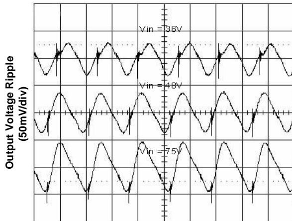
Time - t (2µs/div) Figure 5. Output Ripple Voltage at full Load
