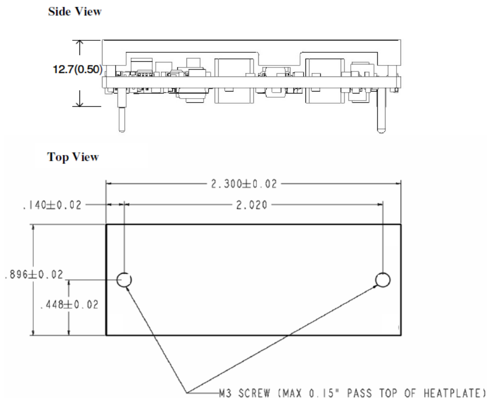
Figure 22. Converter with optional baseplate
