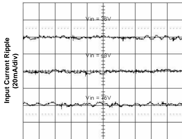
Time - t (1µs/div) Figure 6. Input Reflected Ripple at full Load
