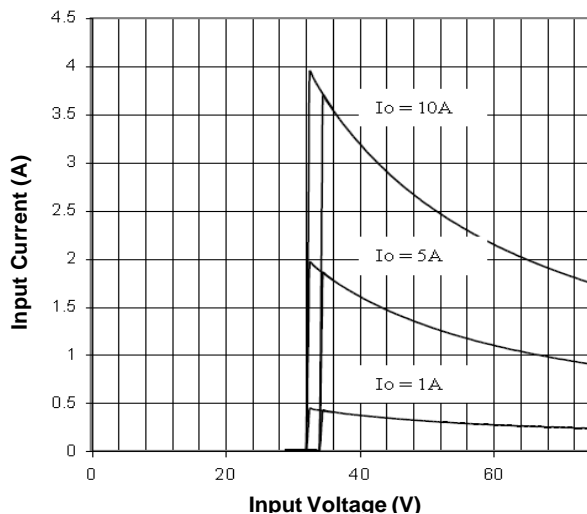
Figure 9. Input Characteristics
