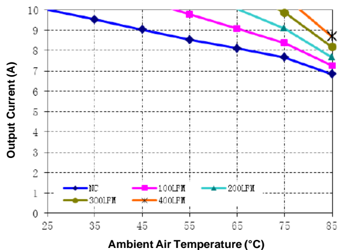
Figure 11. Current Derating Curve for Airflow Direction 3 (Ref. Figure 12 for Airflow Direction; typical Vin, open frame unit)
