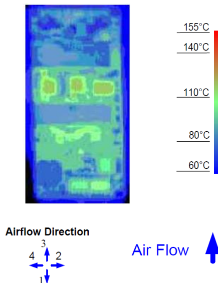
Figure 14. Thermal Image for Airflow Direction 2 (10A output, 55°C ambient, 200 LFM, typical Vin, open frame, socket interface)
