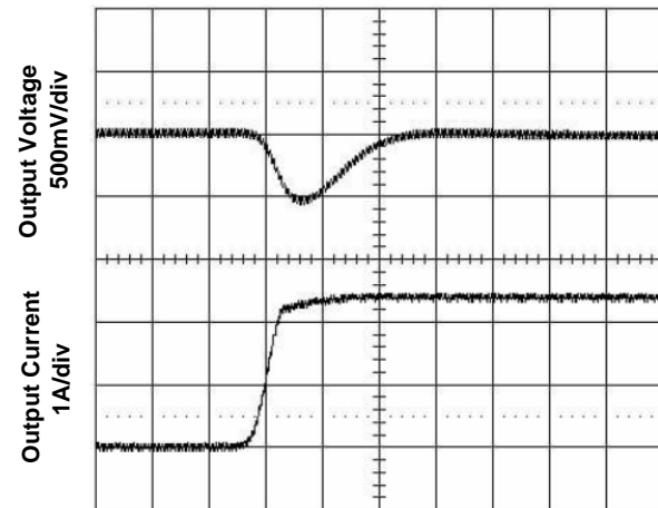
Time - t (50µs/div) Figure 8. Transient Load Response (Typical Vin, load current steps from 50% to 75% at a slew rate 0.1A/µs)
