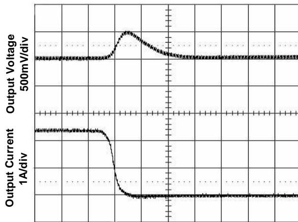
Time - t (50µs/div) Figure 7. Transient Load Response (Typical Vin, load current steps from 50% to 25% at a slew rate 0.1A/µs)
