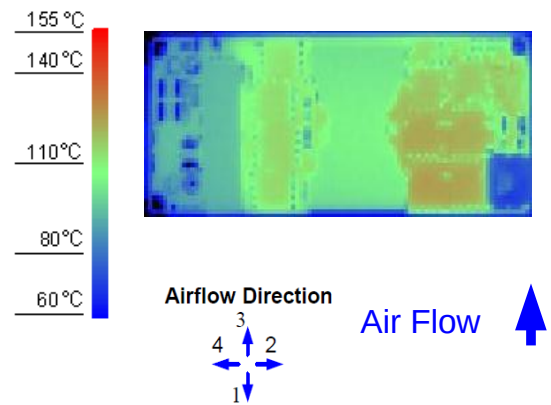
Figure 10. Thermal Image for Airflow Direction 3 (39A output, 55°C ambient, 200 LFM, typical Vin, open frame unit)
