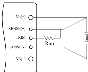
Figure 16. Circuit to Increase Output Voltage
