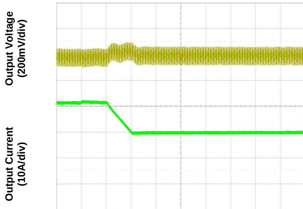
Figure 7. Transient Load Response (typical Vin, load current steps from 75% to 50% at a slew rate 0.1A/ \mu s)
