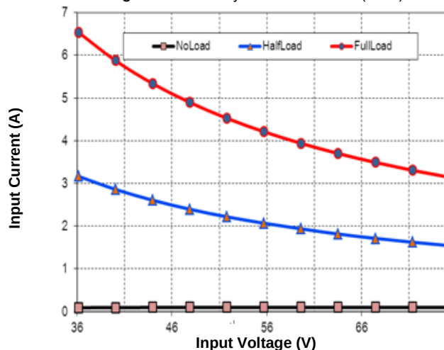
Figure 3. Input Characteristics (25°C)
