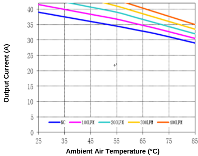
Figure 9. Current Derating Curve for Airflow Direction 3 (Ref. Fig. 10 for Airflow Direction; typical Vin, open frame, solder interface)
