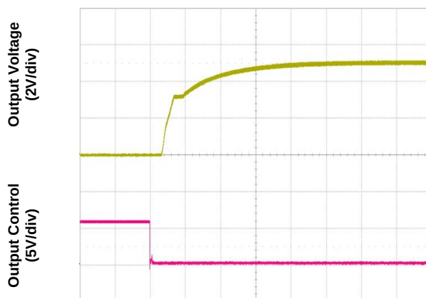
Figure 6. Start-Up from Enable Control
