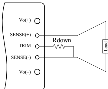
Figure 15. Circuit to Decrease Output Voltage
