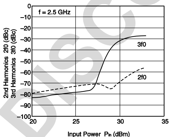
RFC-RF1/RF2 2f 0 , 3f 0 vs. INPUT POWER
