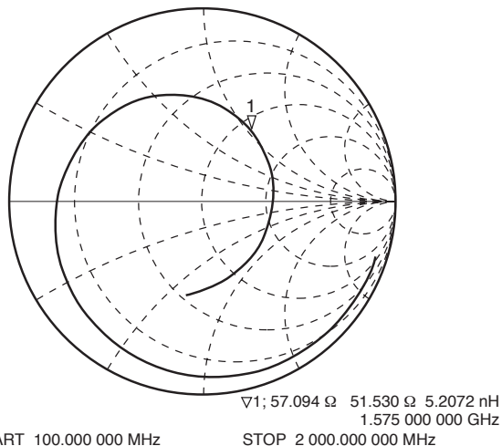
S 11 -FREQUENCY
