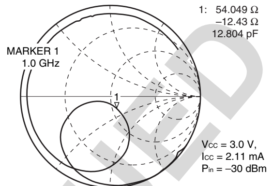
S 22 -FREQUENCY
