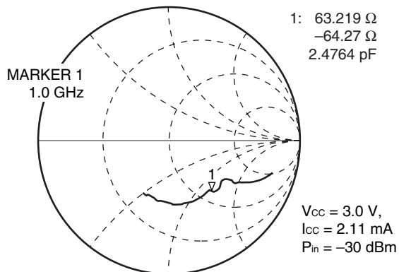
S 11 -FREQUENCY
