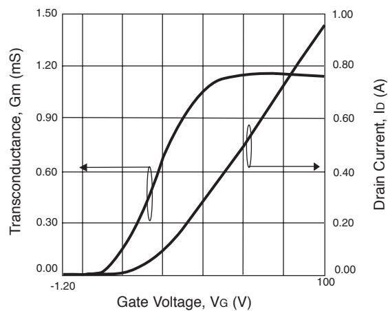
TRANSCONDUCTANCE AND DRAIN CURRENT vs. GATE VOLTAGE
