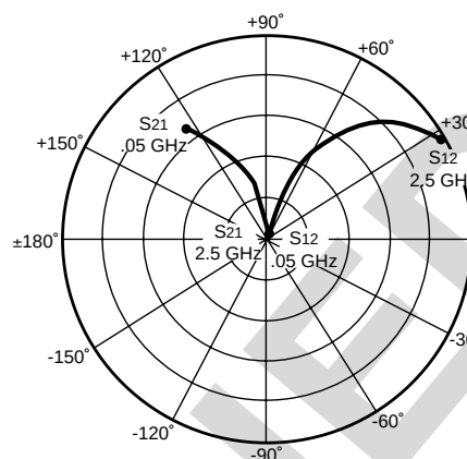
Coordinates in Ohms Frequency in GHz V CE = 5 V, I C = 50 mA
