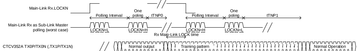
Figure 23. Re-Lock Sequence
