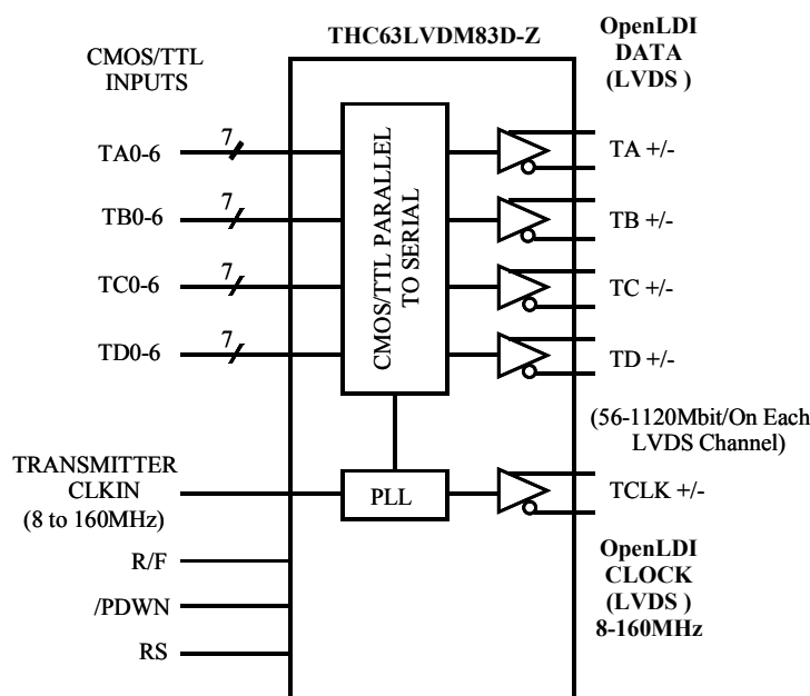
Figure 1. Block Diagram
