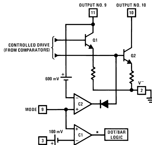
Figure 3. Block Diagram of Mode Pin Function
