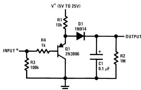
Figure 6. Half-Wave Peak Detector
