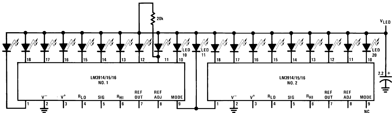
Figure 4. Cascading LM3914/15/16 Series in Dot Mode
