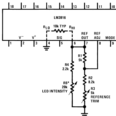
Figure 14. Varying LED Intensity
