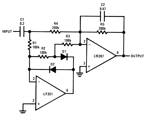
Figure 8. Precision Full-Wave Average Detector
