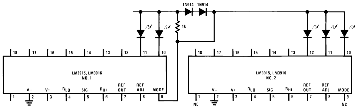
Figure 5. Cascading Drivers in Dot Mode with Pin 1 of Driver #2 Unused
