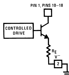
Figure 2. LM3916 Output Circuit
