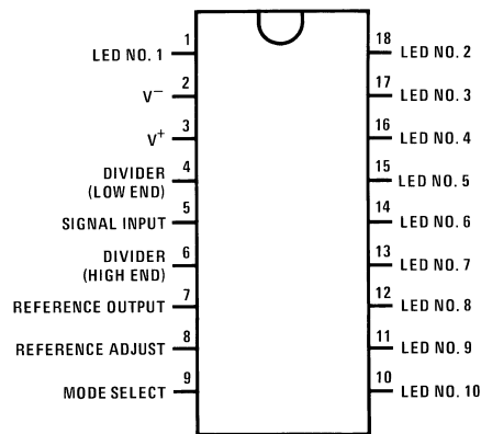
Figure 29. Top View Dual-In-Line Package
