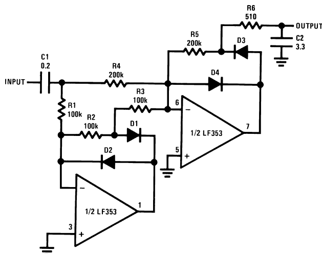
Figure 9. Precision Full-Wave Peak Detector
