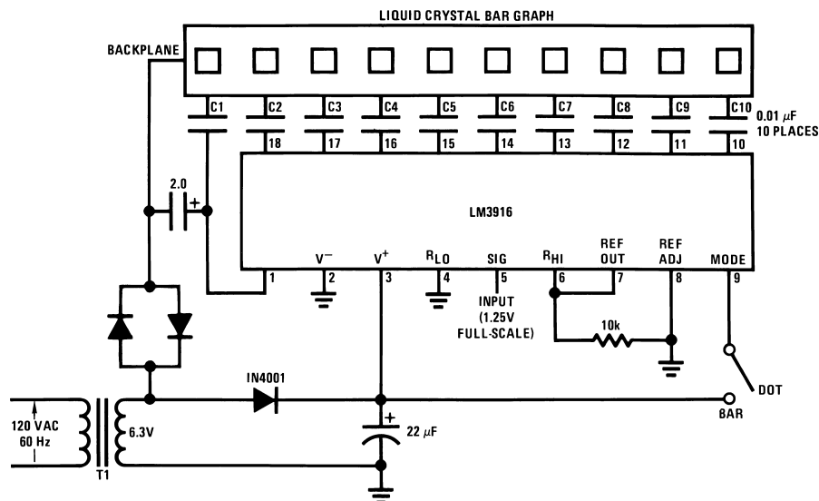
Figure 27. Driving Liquid Crystal Display
