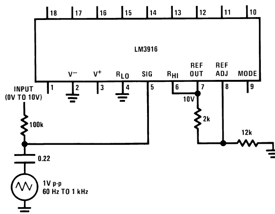
Figure 17. 0V to 10V VU Meter with Smooth Transitions
