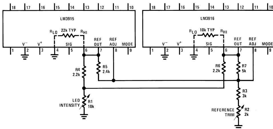
Figure 15. Independent Adjustment of Reference Voltage and LED Intensity for Multiple Drivers
