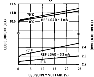
LED Driver Current Regulation
