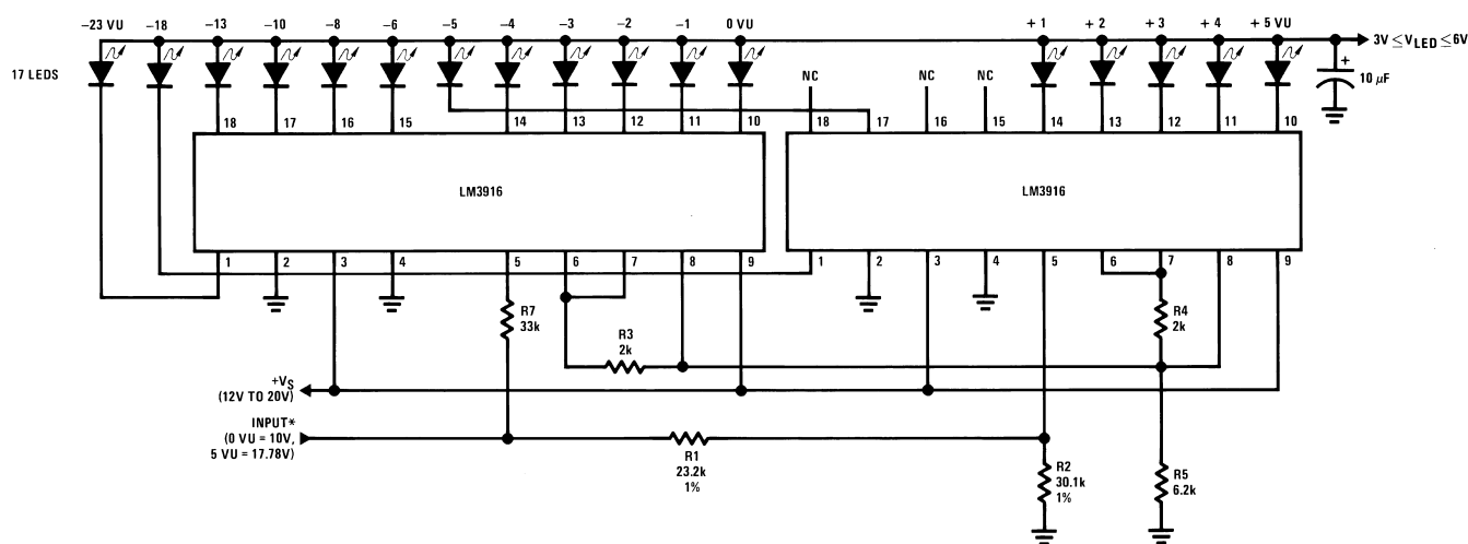
Figure 21. Indicator and Alarm, Full-Scale Changes Display From Dot to Bar
