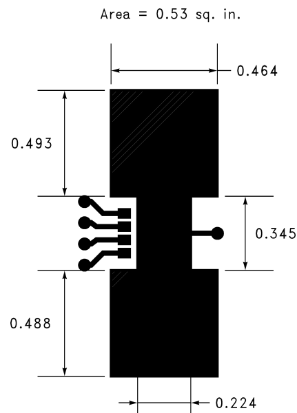
Figure 12. SCENARIO D, \theta_{JA} = 83^{\circ}\text{C/W}
