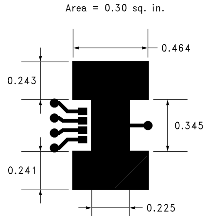
Figure 11. SCENARIO C, \theta_{JA} = 92^{\circ}\text{C/W}
