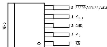
Figure 3. Top View TO263-5 Package
