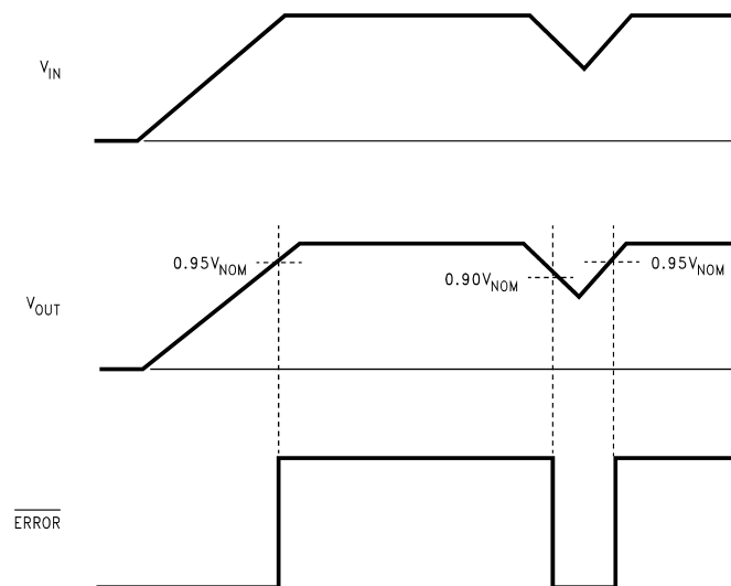
Figure 4. \overline{\text{Error}} Flag Operation
