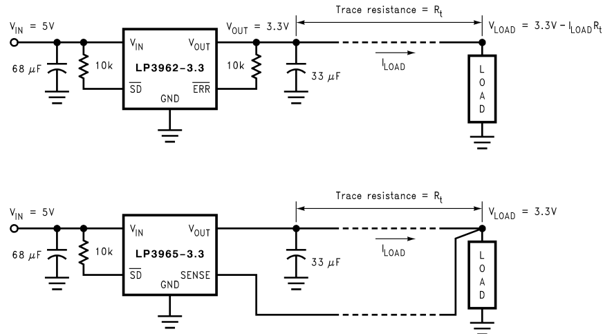
Figure 5. Improving remote load regulation using LP3965
