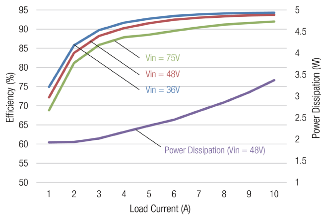
UEE-5/10-D48 Efficiency and Power Dissipation @ Ta= +25° C
