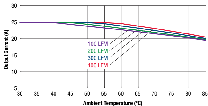
UEE-3.3/25-D48 Maximum Current Temperature Derating at Sea Level ( V_{in} = 48\text{V} , with baseplate. Airflow direction is from Vin to Vout.)
