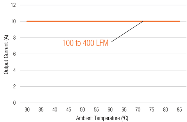
UEE-5/10-D48 Maximum Current Temperature Derating at Sea Level (Vin=48V, no baseplate, airflow is from Vin to Vout)
