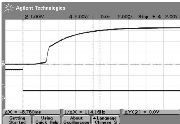
On/Off Enable Delay (Vin=48V, Vout=nom., Iout=0A, Clad=0, Ta=+25° C., ScopeBW=20Mhz, Trace 2=Vout, Trace 4=Enable.
