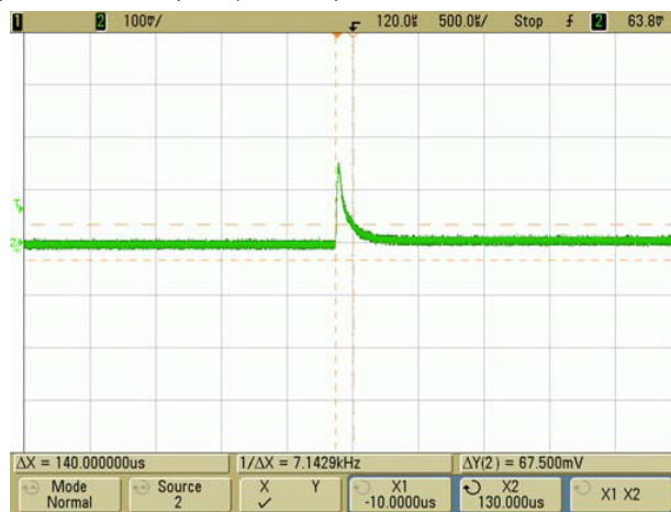
Step Load Transient Response (Slew=1A / \mu Sec., Vin=48V., Clad=0, Iout=15A to 22.5A)
