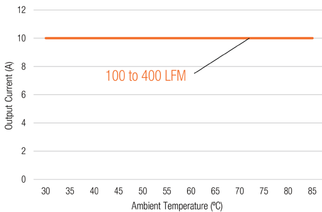
UEE-5/10-D48 Maximum Current Temperature Derating at Sea Level (Vin=48V, no baseplate, airflow is from +Vin to -Vin)
