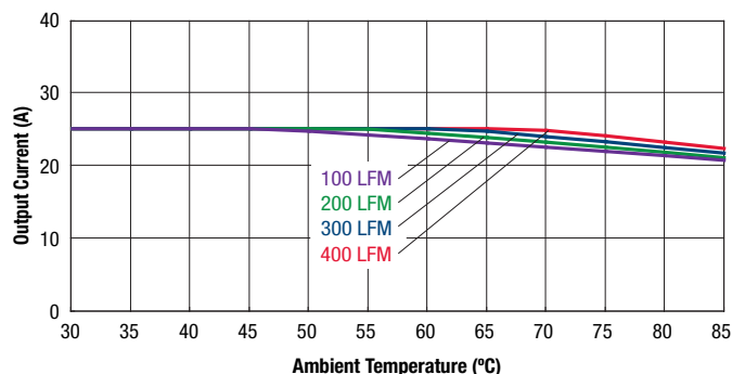
UEE-3.3/25-D48 Maximum Current Temperature Derating at Sea Level ( V_{in} = 48\text{V} , with baseplate. Airflow direction is transverse from +Vin to -Vin.)
