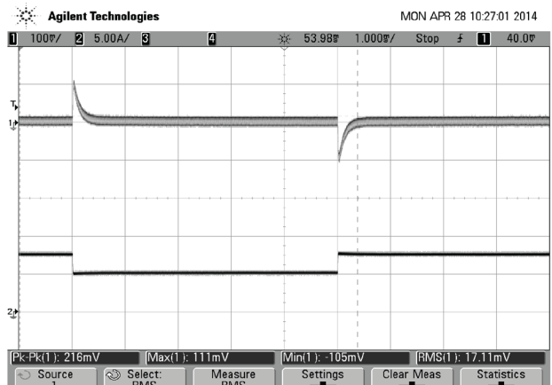
Step Load Transient Response (Vin=48V, Vout=nom., Load=220uF, Iout=75 to 50 to 75% of full load, Ta=25° C) Trace 1=Vout, 100mV/div., 1mS/div.
