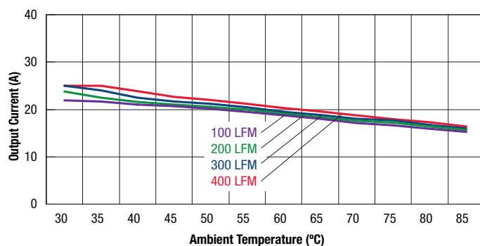
UEE-3.3/25-D48 Maximum Current Temperature Derating at Sea Level ( V_{in} = 48\text{V} , no baseplate. Airflow direction is longitudinal, from Vin to Vout.)
