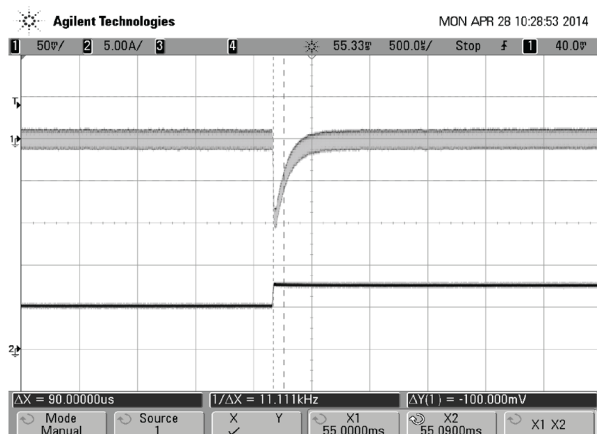
Step Load Transient Response (Vin=48V, Vout=nom., Load=220uF, Iout=50% to 75% of full load, Ta=25° C) Trace 1=Vout, 50mV/div., 500uS/div.
