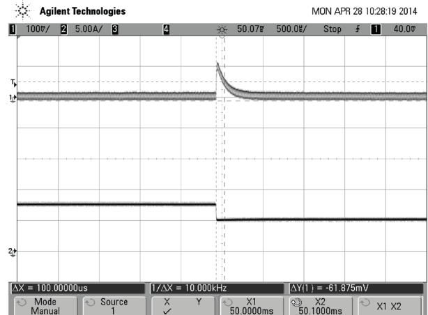
Step Load Transient Response (Vin=48V, Vout=nom., Load=220uF, Iout=75% to 50% of full load, Ta=25° C) Trace 1=Vout, 100mV/div., 500uS/div.
