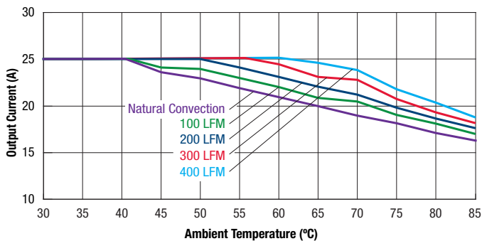
UEE-3.3/25-D48 Maximum Current Temperature Derating at Sea Level ( V_{in} = 48\text{V} , no baseplate. Airflow direction is transverse.)
