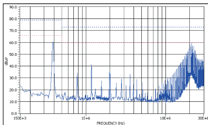
Graph 8. Conducted emissions performance, Negative Line, CISPR 22, Class A, full load
