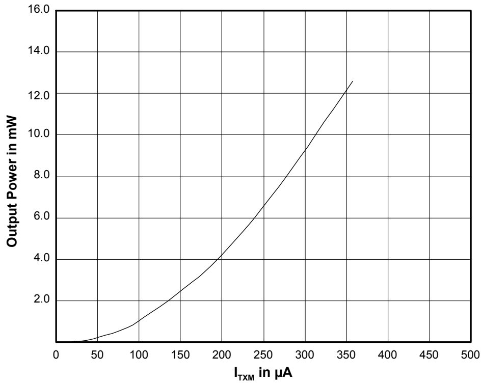
TR8001 R 1 Output Power vs I TXM
