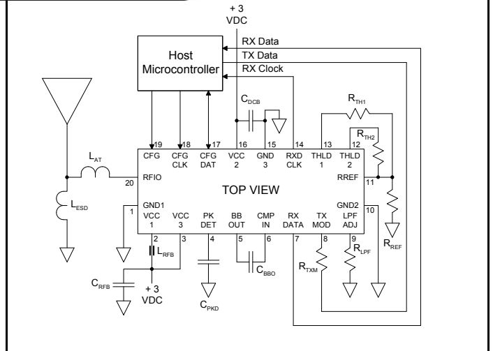
Transceiver Application Circuit ASK Configuration
