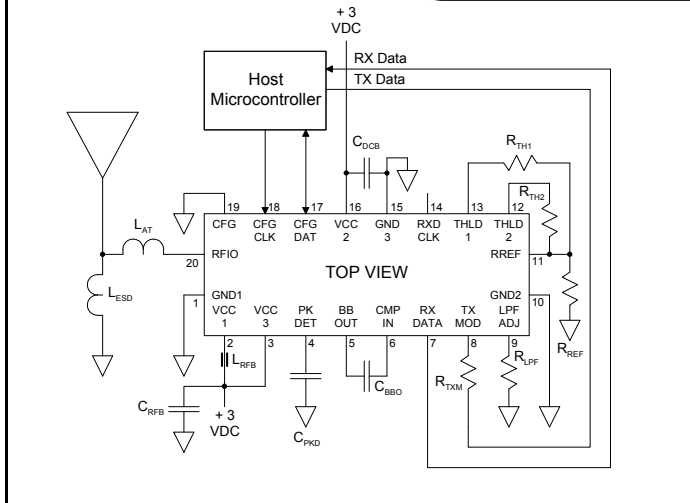
3G ASH Transceiver Application Circuit 2G Default OOK/ASK Configuration
