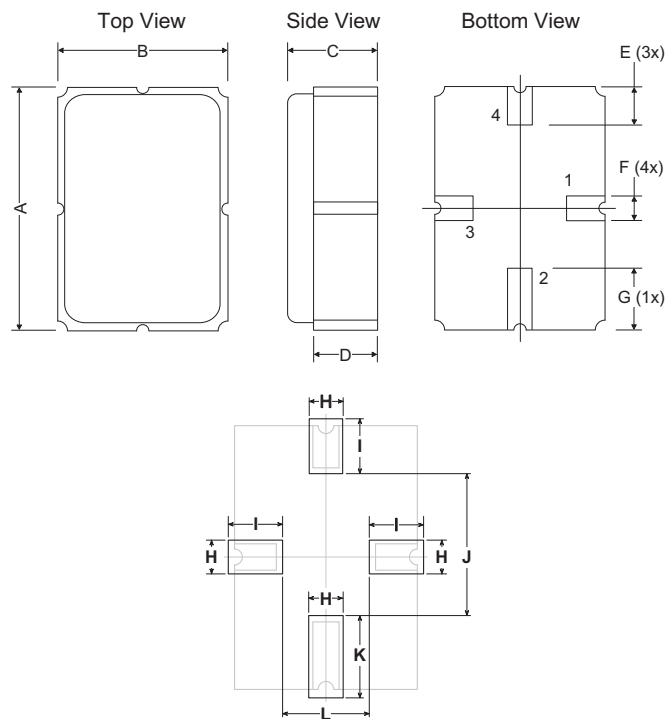
PCB Land Pattern Top View
