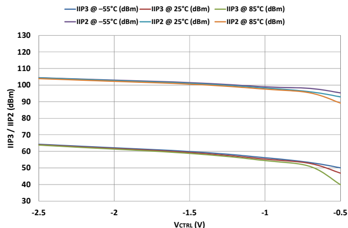
Figure 12. IIP3 / IIP2 vs. V_{CTRL} Over Temperature
