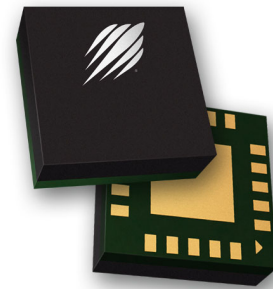
Figure 2. Package Type 20-lead 4 × 4 mm LGA
