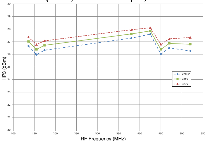
Figure 12. IIP3 vs Voltage (25 °C, -6dBm LO Input, 109.65 MHz IF)
