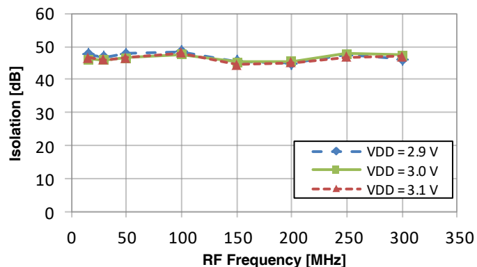
Figure 25. RF to IF Isolation vs V_{DD}
