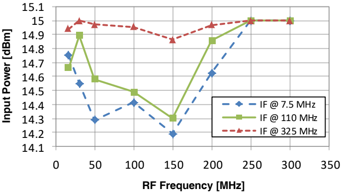
Figure 43. P1dB vs IF Frequency (25 °C, -8 dBm LO Input)
