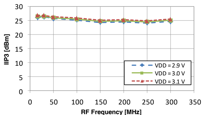
Figure 29. IIP3 vs V_{DD}
