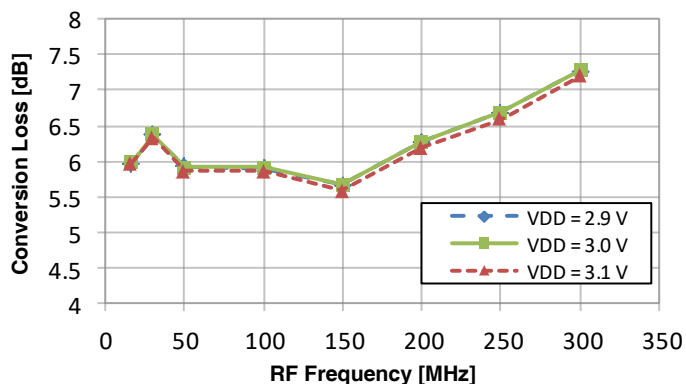
Figure 24. Conversion Loss vs V_{DD}
