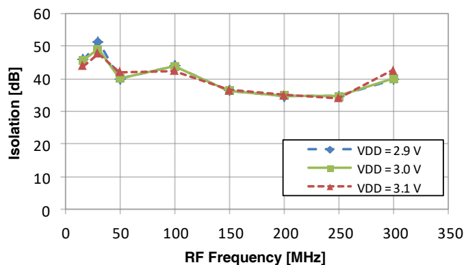
Figure 26. LO to IF Isolation vs V_{DD}
