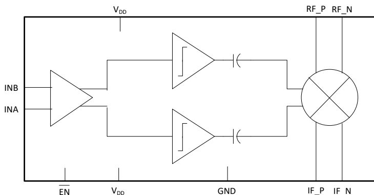
Figure 1. Functional Diagram
