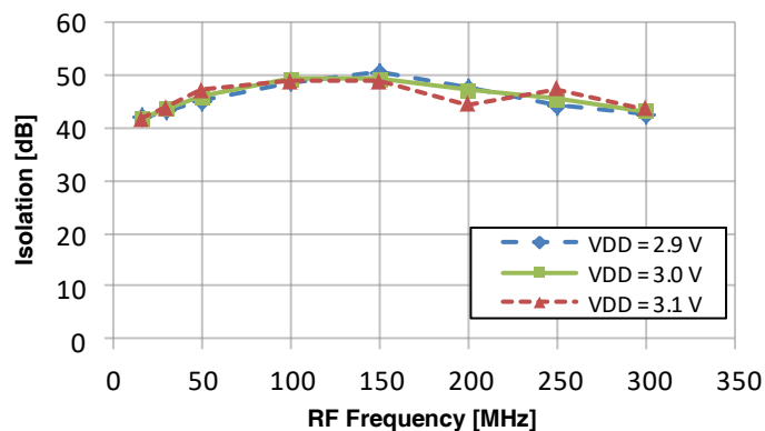
Figure 27. LO to RF Isolation vs V_{DD}
