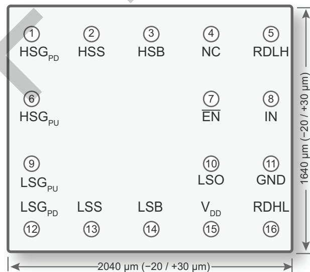
Figure 11 • Pin Layout for PE29100 (1)(2)
