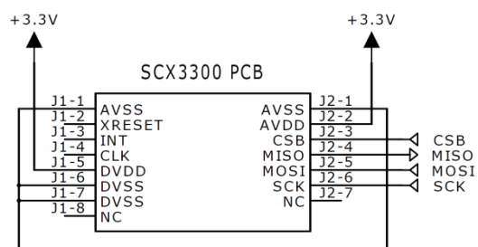
Figure 1. SCx3300 PCB pinout and external connections.
