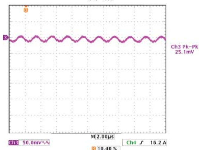
Output Ripple and Noise( V_{in}=12V , V_{out}=3.3V , I_{out}=0A , C_{out}=100\mu f , T_a=+25^{\circ}C ) Ch3=Vout
