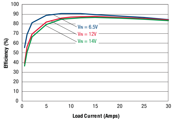
Efficiency vs. Line Voltage and Load Current @ +25°C. (Vout = 1.0V)
