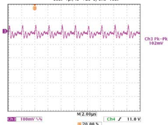
Output Ripple and Noise( V_{in}=12V , V_{out}=3.3V , I_{out}=25A , C_{out}=100\mu f , T_a=+25^{\circ}C ) Ch3=Vout
