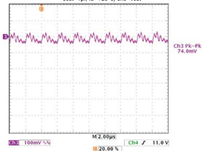
Output Ripple and Noise( V_{in}=12V , V_{out}=0.6V , I_{out}=0A , C_{out}=1\mu f , T_a=+25^{\circ}C ) Ch3=Vout
