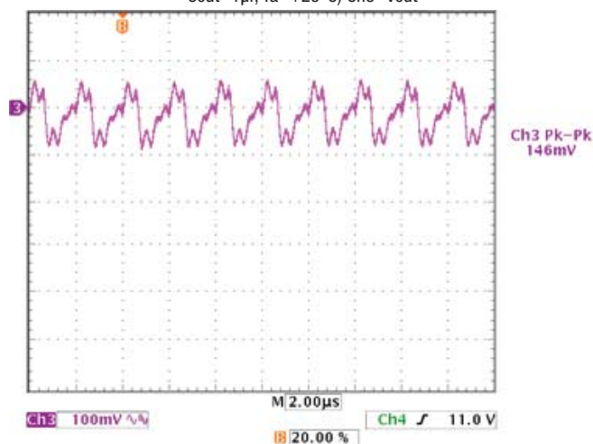
Output Ripple and Noise( V_{in}=12V , V_{out}=0.6V , I_{out}=25A , C_{out}=1\mu f , T_a=+25^{\circ}C ) Ch3= V_{out}
